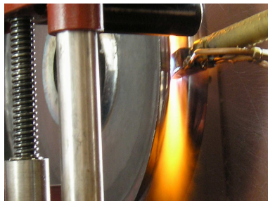
Flame Hardened wireline grooves for longer rope and sheave life
